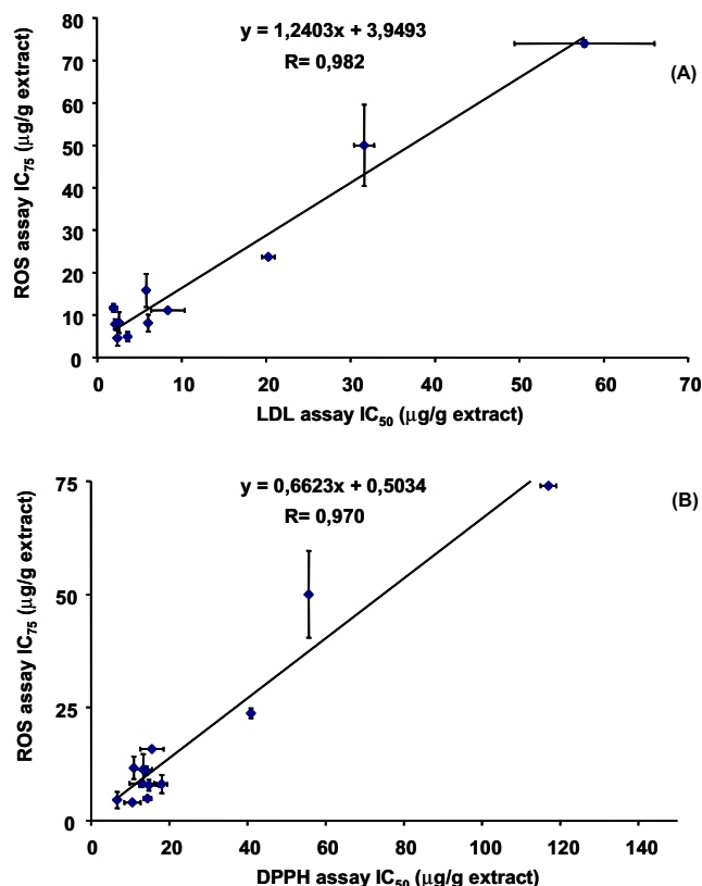
Fig. 2. Linear regression analysis between: (A) LDL oxidation and intracellular ROS assays and (B) DPPH radical scavenging and intracellular ROS assays.
