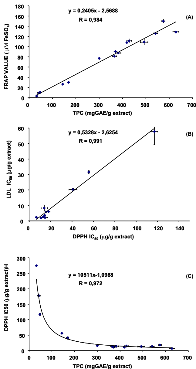
Fig. 1. Linear regression analysis between: (A) total polyphenolic content (TPC) and FRAP assays; (B) DPPH radical scavenging and LDL oxidation assays and (C) TPC and DPPH radical scavenging assays.
