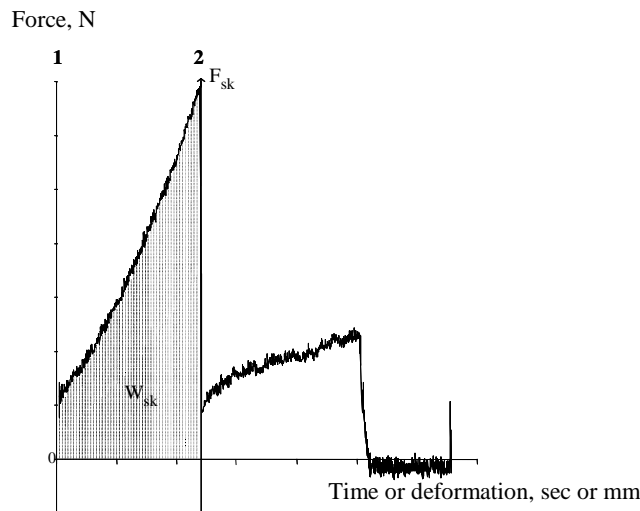
Figure2 Force-time (deformation) curve corresponding to the berry skin puncture test
