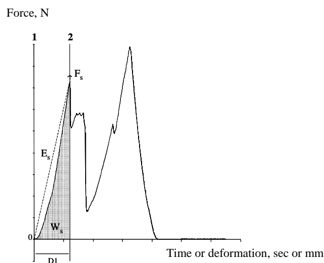
Figure3 Force-distance curve related to the test for seed hardness determination
